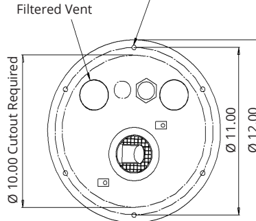
Hopper Mounted
